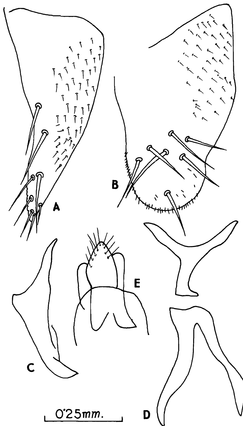
Text-fig. 1 A-E, Cicadella spectra (Distant) ; A, Male plate ; B, Pygofer; C, style; D, Aedeagus; E, Anal tube.
