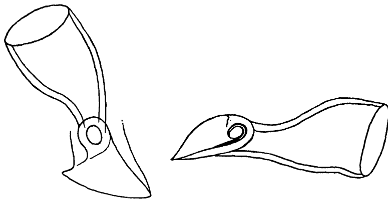
TEXT-FIG. 2.— Limnodrilus sp. ; chitinous penis sheaths, one drawn from one side, the other from the other side of the body.
