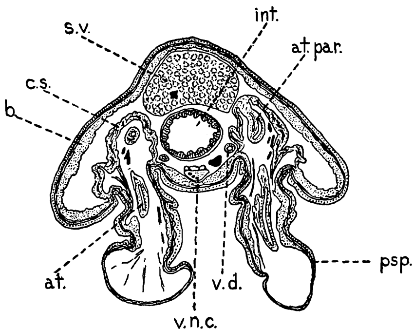
TEXT-FIG. 1.— Branchiura sowerbyi ; transverse section through segm. xi, to show everted pseudopenes ; \times 34 (Abbe's drawing apparatus). At. , atrium within coelomic sac ; at. par. , atrium and paratrium together, before union, just after entering coelomic sac ; b. , body-wall, with the three layers, epithelium, circular and longitudinal muscular coats ; c.s. , muscular wall of coelomic sac, which by its contraction causes extrusion of pseudopenis ; int. , intestine ; psp. , pseudopenis, the everted ectal portion of atrium ; s.v. , seminal vesicle (sperm sac) containing sperm morulae ; v.d. , vas deferens ; v.n.c. , ventral nerve cord.
