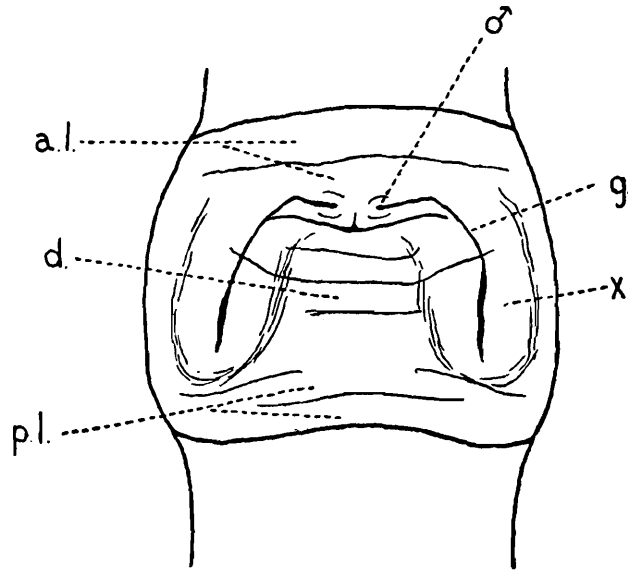
TEXT-FIG. 3.— Notoscolex choprai ; the male area. A.l. , anterior lip, with transverse groove; d. , central depression; g. , groove leading to male pore, ♂; p.l. , posterior lip, also with transverse groove; x. , lateral lip around posterior end of groove (forming almost an independent papilla).
