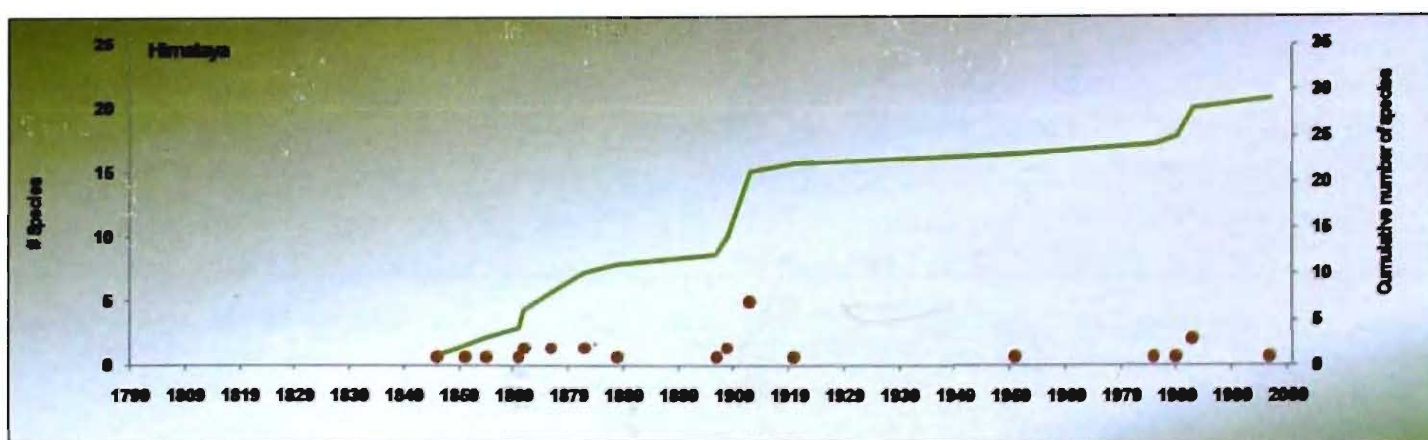
Figure 6. Pattern of species discovery of Amphibia in Himalaya (dots indicate discovery and line indicates cumulative discovery pattern).
