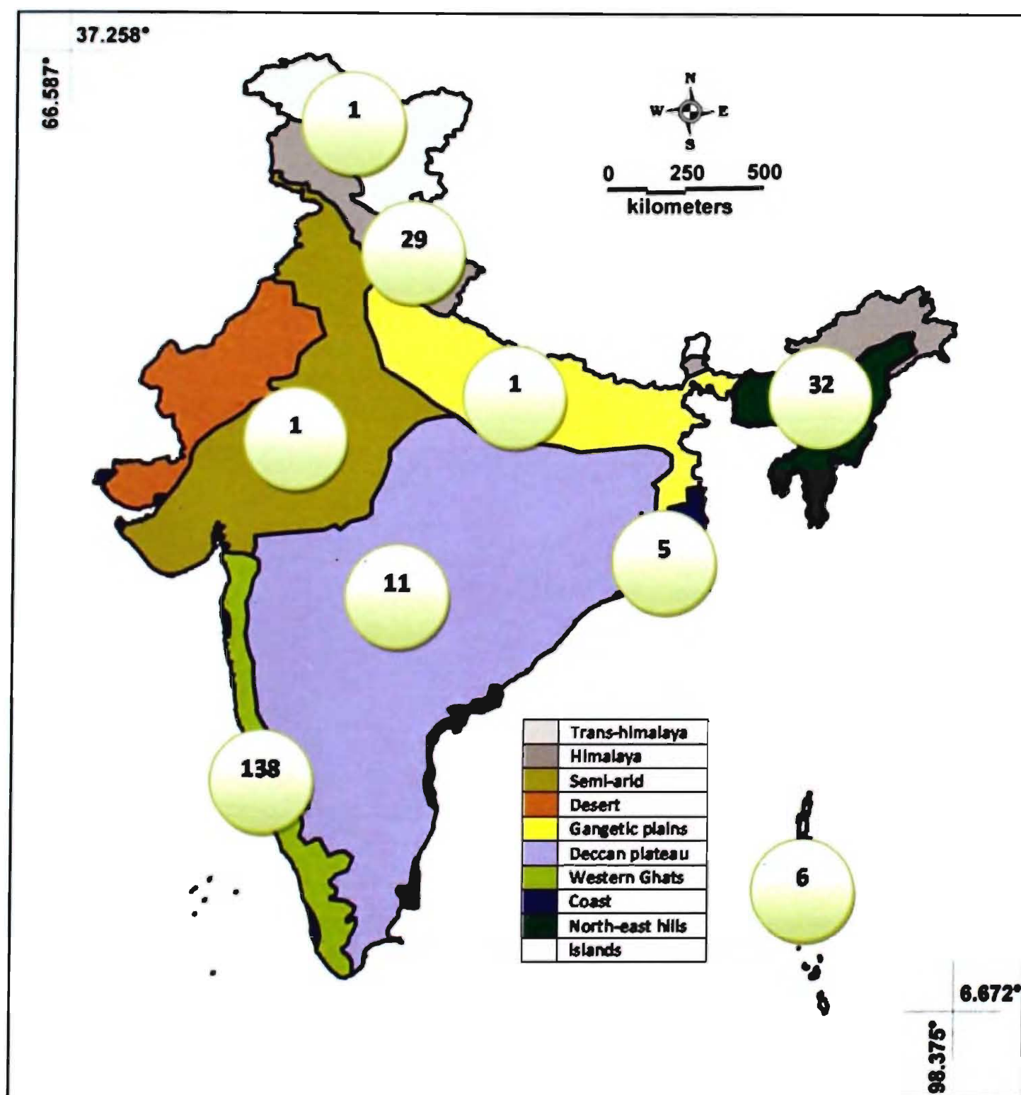
Figure 3. Number of amphibian species with type localities known from the various biogeographic zones of India.
