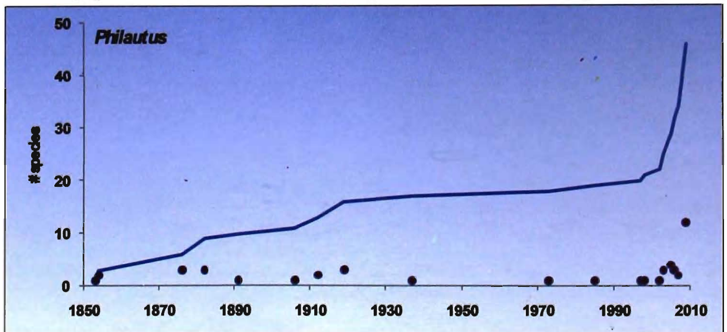
Figure 11. Pattern of species discoveries in the genus Philautus (dots indicate discovery and line indicates cumulative discovery pattern).
