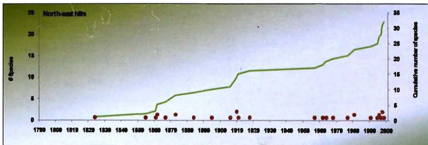
Figure 5. Pattern of species discovery of Amphibia in North-east Hills (dots indicate discovery and line indicates cumulative discovery pattern).
