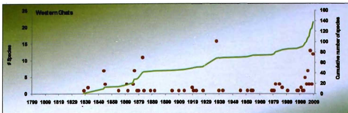
Figure 4. Pattern of species discovery of Amphibia in Western Ghats (dots indicate discovery and line indicates cumulative discovery pattern).
