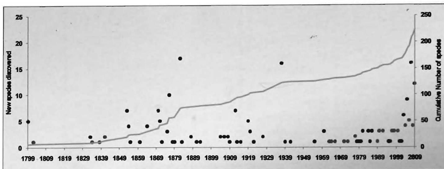
Figure 1. Pattern of species discovery of Amphibia in India (dots indicate discovery and line indicates cumulative discovery pattern).
