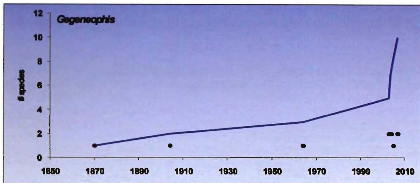
Figure 12. Pattern of species discoveries in the genus Gegeneophis (dots indicate discovery and line indicates cumulative discovery pattern).
