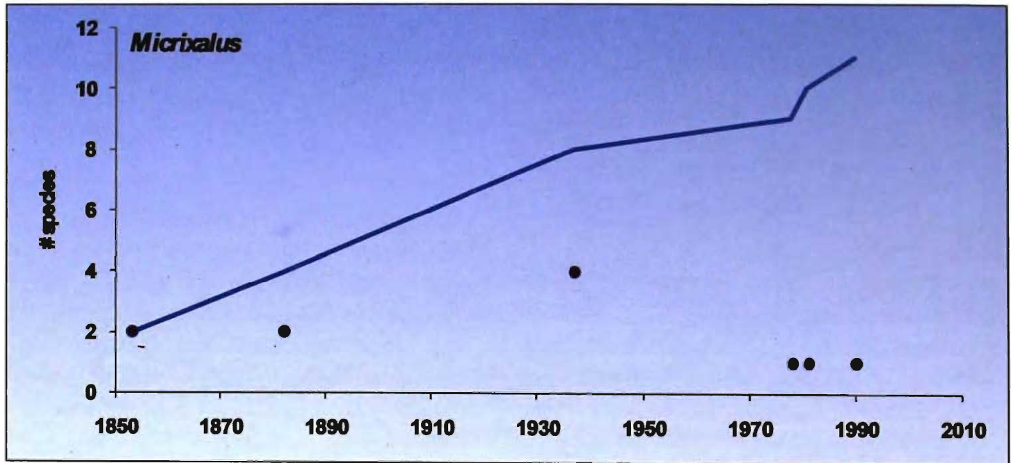
Figure 10. Pattern of species discoveries in the genus Micrixalus (dots indicate discovery and line indicates cumulative discovery pattern).
