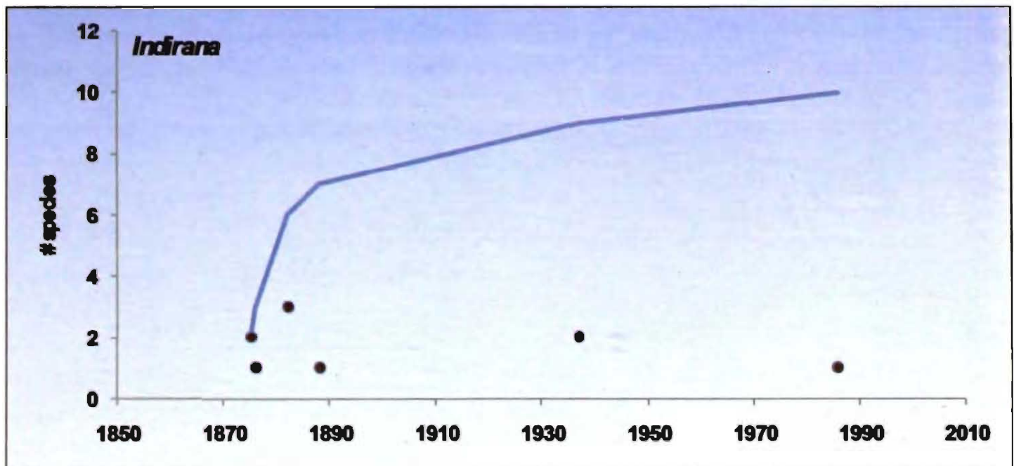
Figure 9. Pattern of species discoveries in the genus Indirana (dots indicate discovery and line indicates cumulative discovery pattern).
