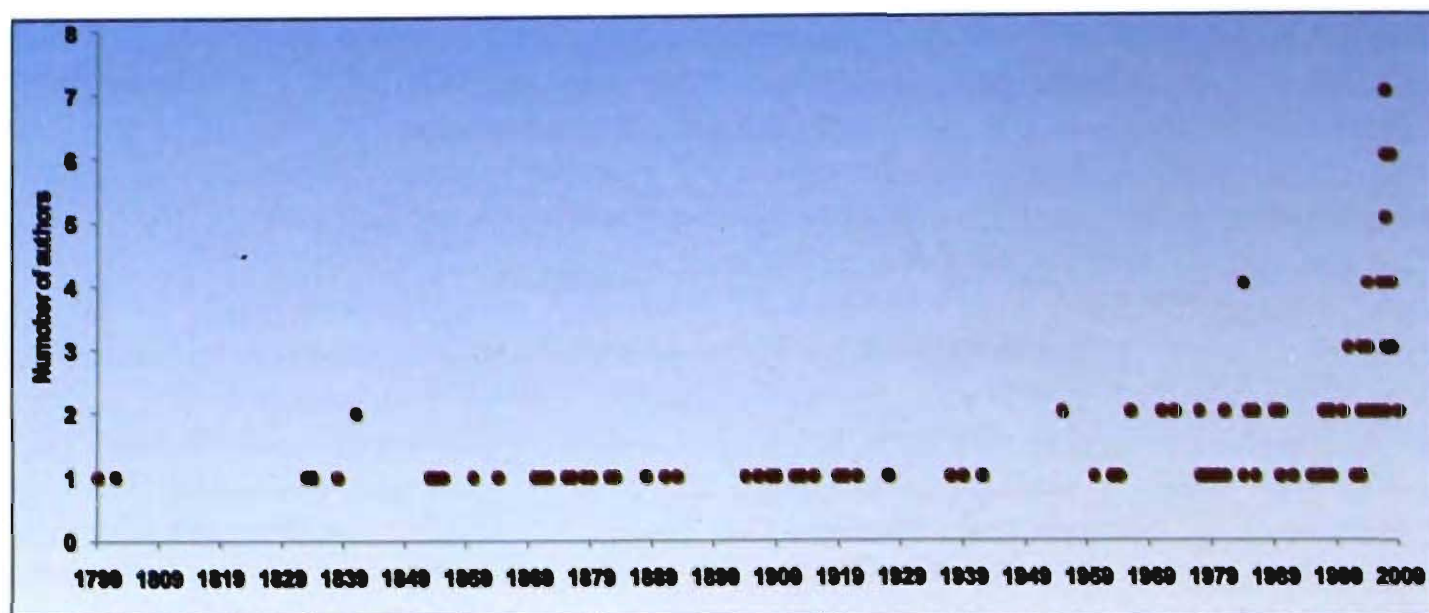
Figure 2. Single vis-à-vis multiple authorship in species descriptions from India
