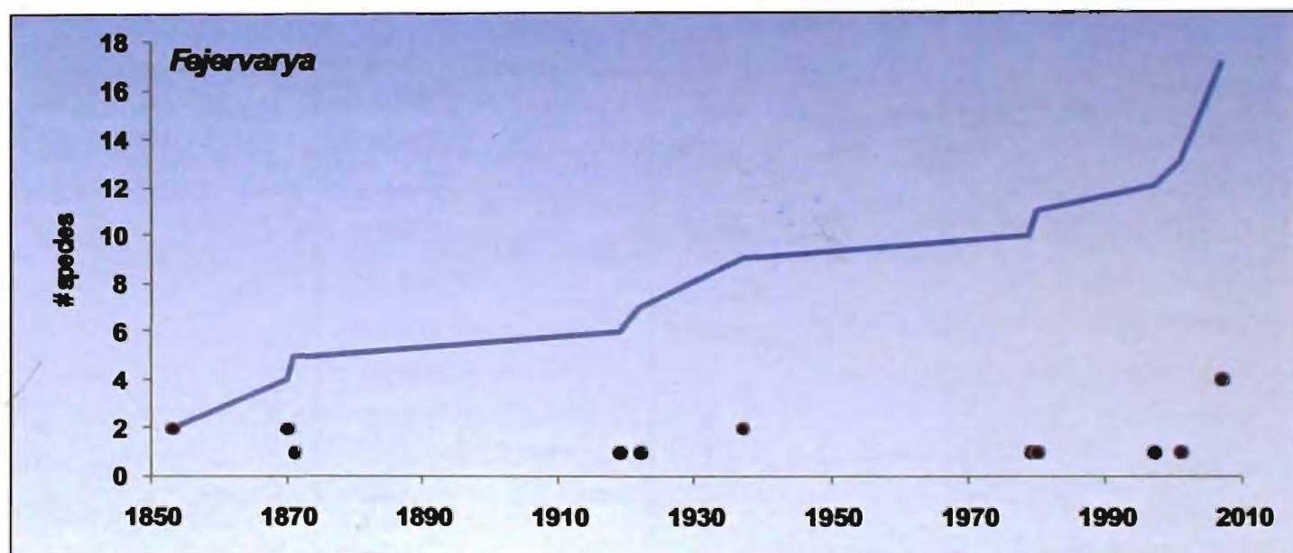
Figure 7. Pattern of species discoveries in the genus Fejervarya (dots indicate discovery and line indicates cumulative discovery pattern).
