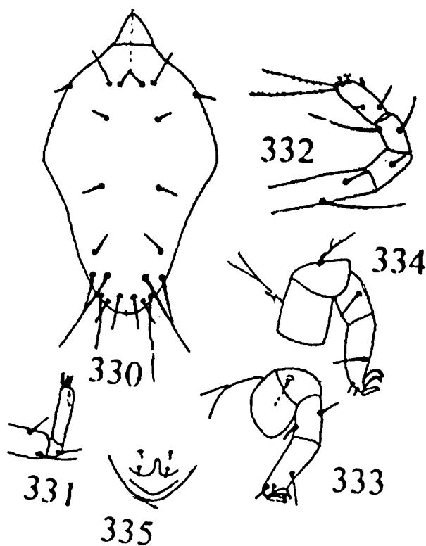
Figs. 325-335 : Parapronematus cameliae Gupta (female) : 325. Dorsal view, 326. Palp, 327. Tibia and tarsus of leg III, 328. Tibia and tarsus of leg IV, 329. Anal region. (after Gupta, 1992); Parapronematus ferox Gupta (female) : 330. Dorsal view, 331. Palp, 332. Leg I, 333. Leg III, 334. Leg IV, 335. Genital region. (after Gupta, 1991)
