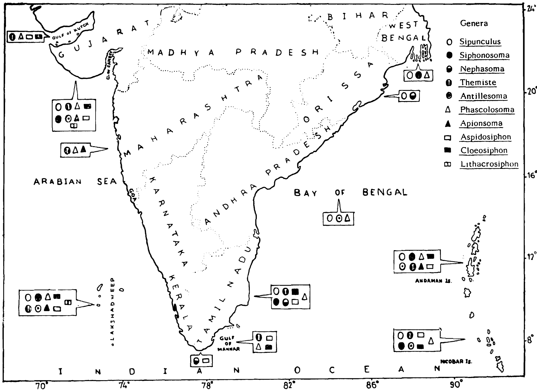
Fig. 203. The geographical distribution of the genera of sipunculans in the Indian coast.
