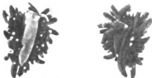
FIG. 1.—Photographs of the ventral and dorsal views of the type-specimen of Stiliger pica Annandale & Prashad (magnified).
